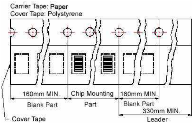
Tape Material
