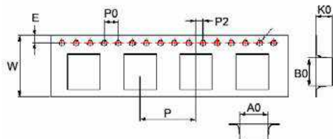
Tape Dimensions
