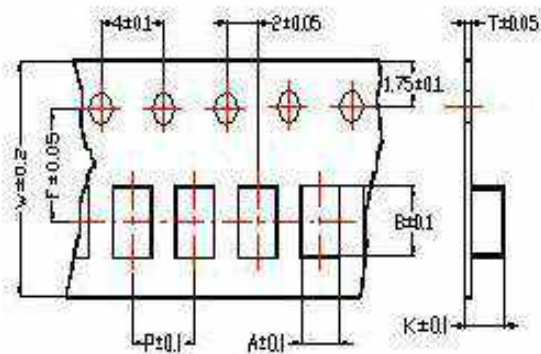
Tape Dimensions
