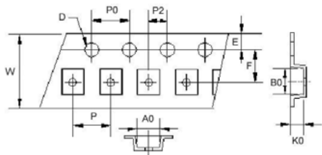
Tape Dimensions
