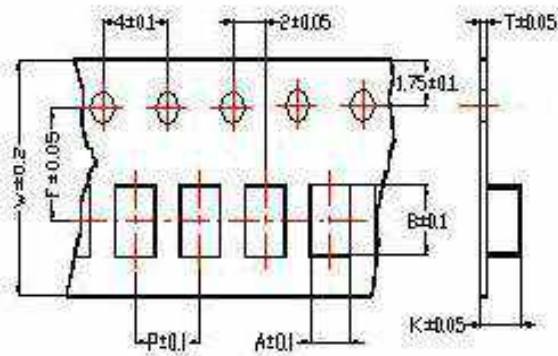
Tape Dimensions
