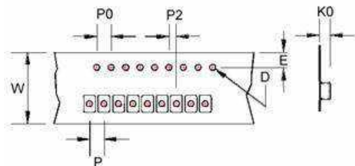
Tape Dimensions
