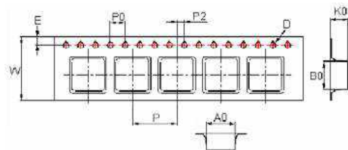
Tape Dimensions
