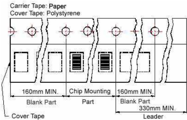
Tape Material
