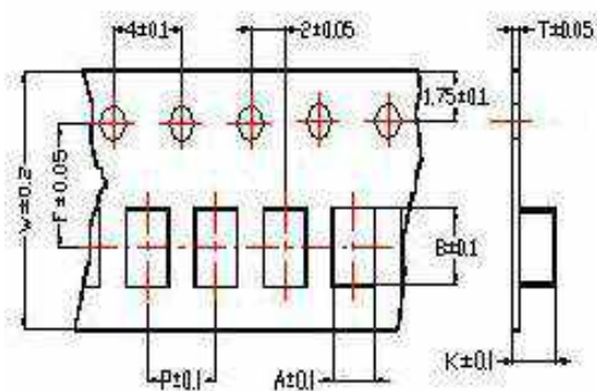
Tape Dimensions
