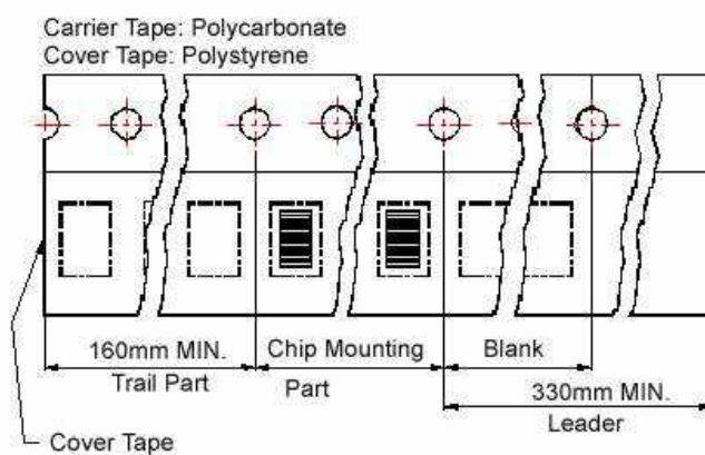
Tape Material
