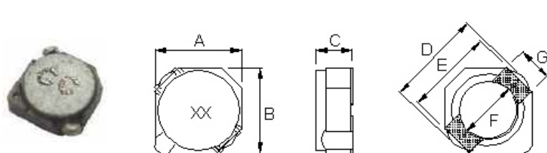
Dimension in mm
