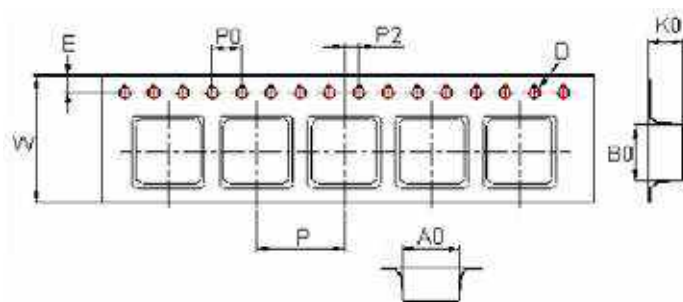
Tape Dimensions
