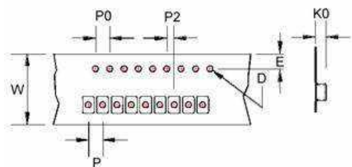
Tape Dimensions
