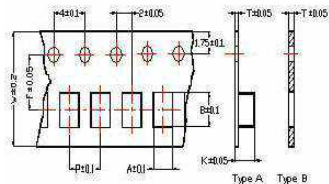
Tape Dimensions
